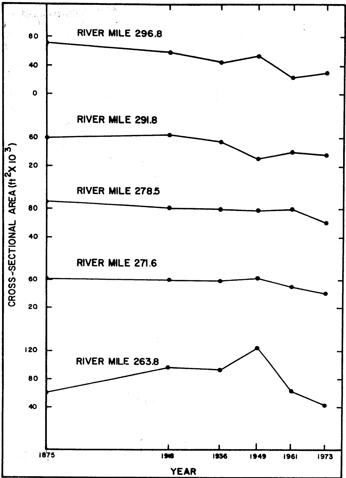
FIGURE A-5-8. LWRP area of the Mississippi River at river miles 296.8, 291.8, 278.5, 271.6 and 263.8 between 1875 and 1974.
