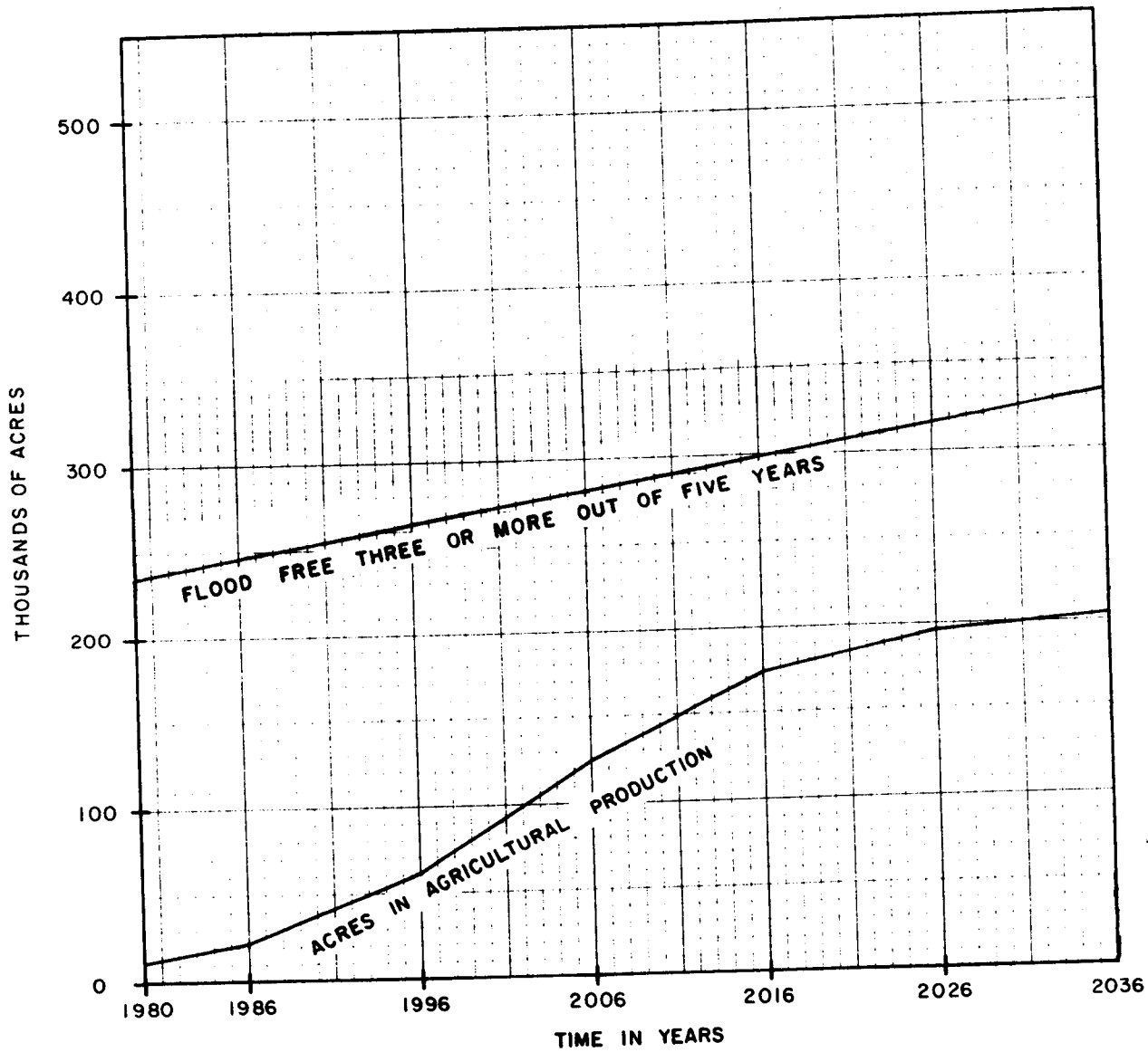
FIGURE D-2-1 MOST PROBABLE FUTURE WITHOUT PROJECT LOWER ATCHAFALAYA BASIN FLOODWAY
