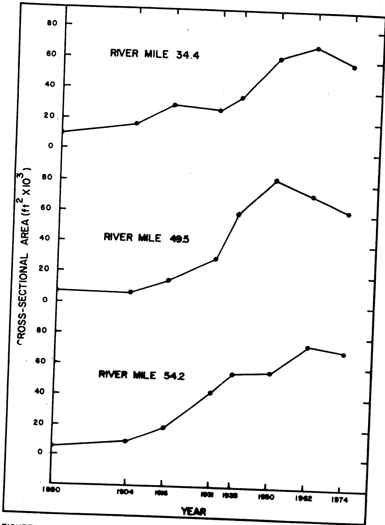
FIGURE A-5-5. LWRP area of the Atchafalaya River at river miles 34.4, 49.4 and 54.2 between 1880 and 1974.
