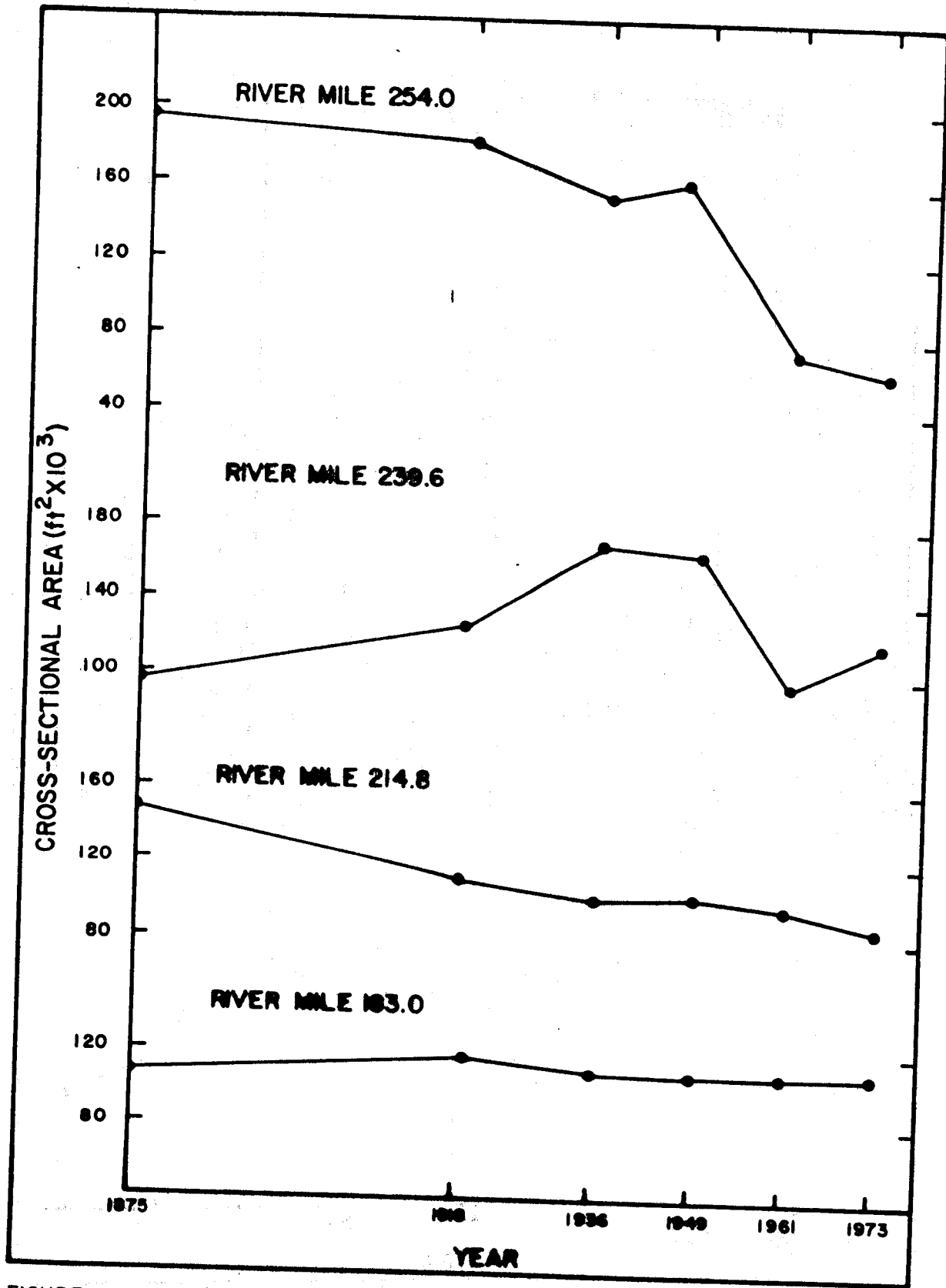
FIGURE A-5-9. LWRP area of the Mississippi River at river miles 254.0, 239.6, 214.8 and 183.0 between 1875 and 1974.
