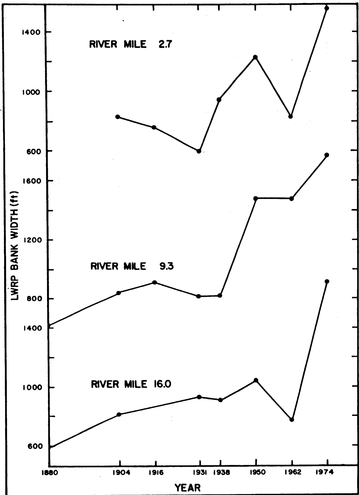
FIGURE A-5-2. LWRP bank widths of the Atchafalaya River at river miles 2.7, 9.3 and 16.0 between 1880 and 1974.
