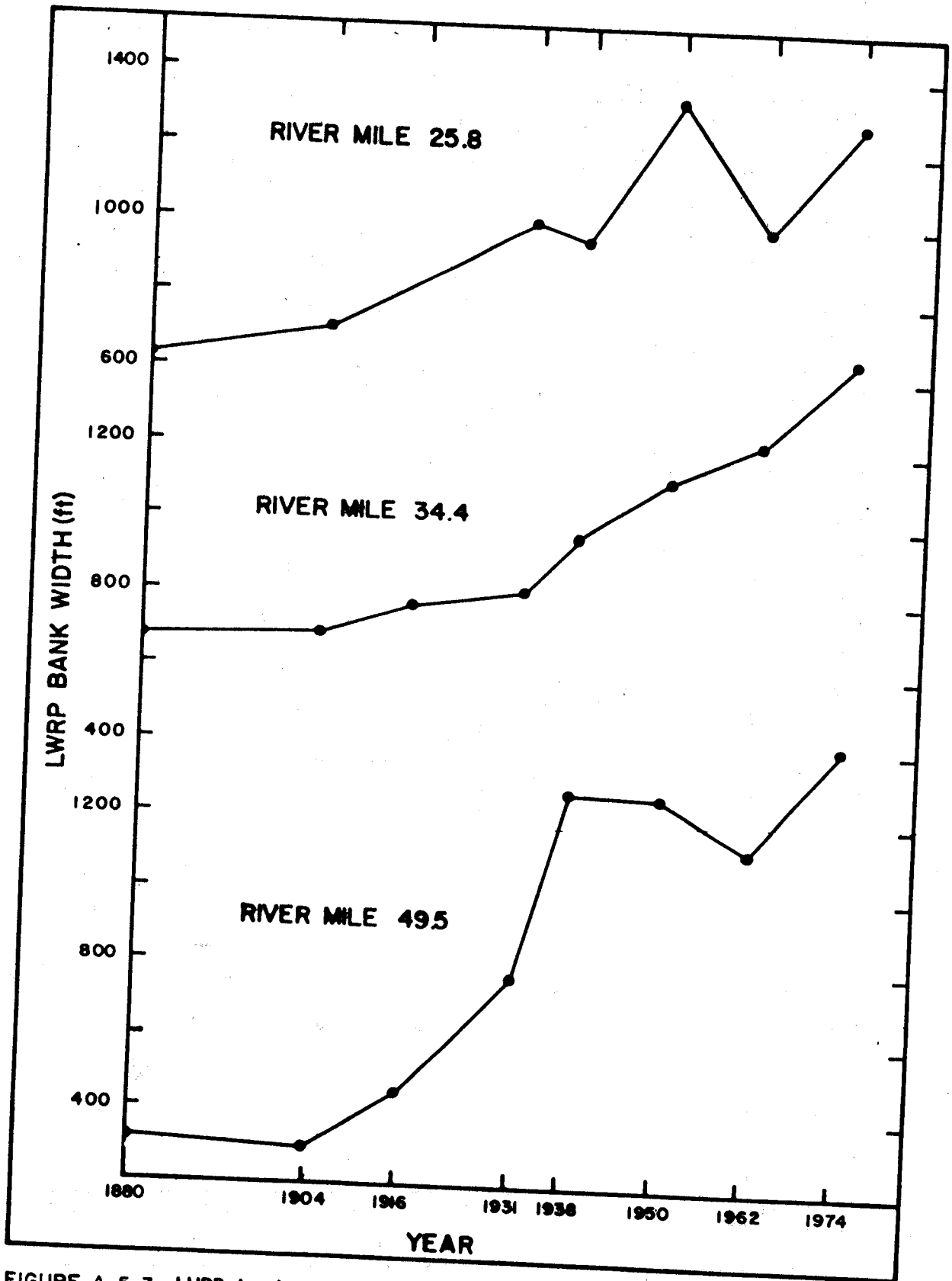
FIGURE A-5-3. LWRP bank widths of the Atchafalaya River at river miles 25.8, 34.4 and 49.5 between 1880 and 1974.
