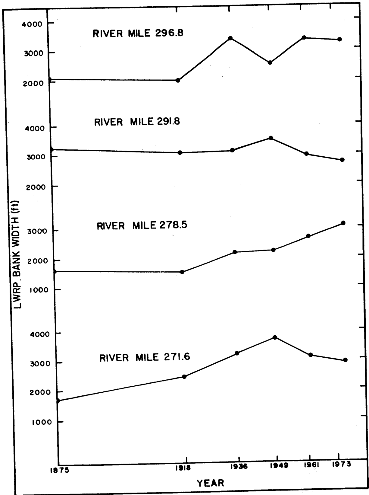
FIGURE A-5-6. LWRP bank widths of the Mississippi River at river miles 296.8, 291.8, 278.5 and 271.6 between 1875 and 1974.
