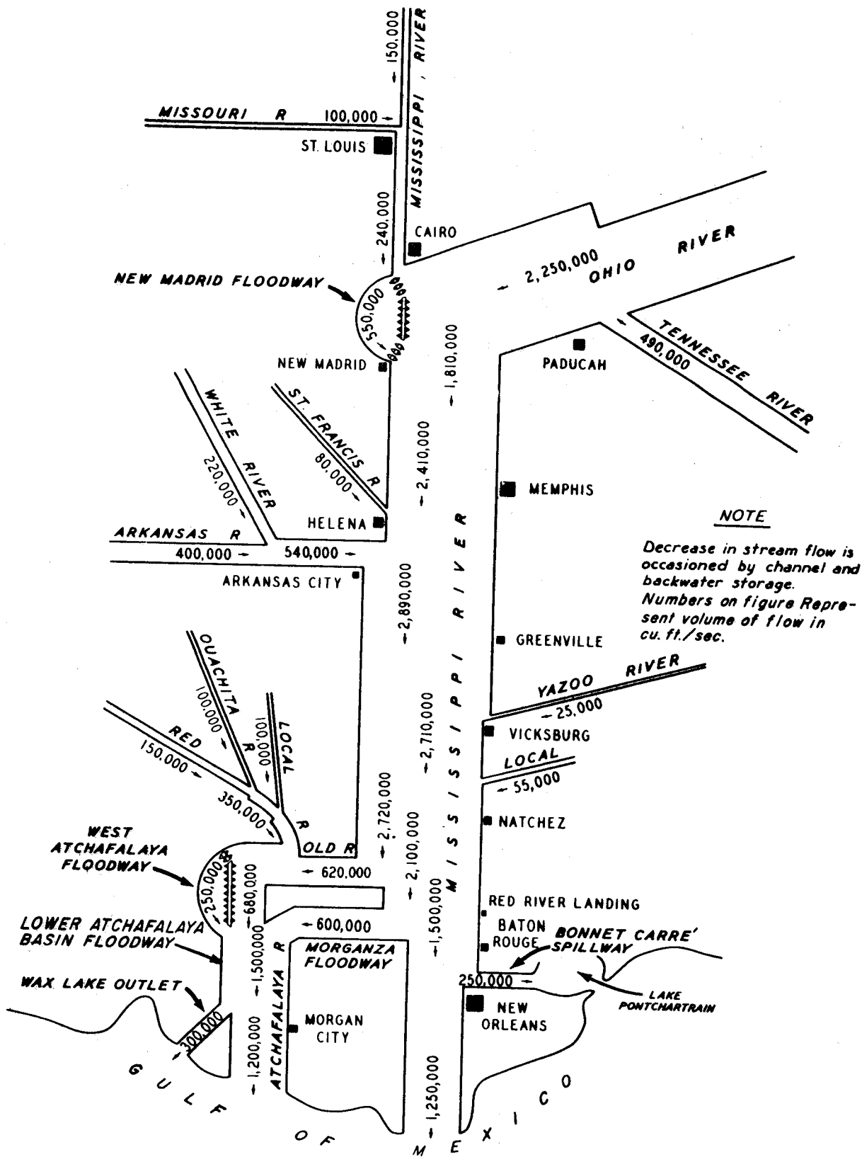
FIGURE A-4-1 PROJECT DESIGN FLOOD
