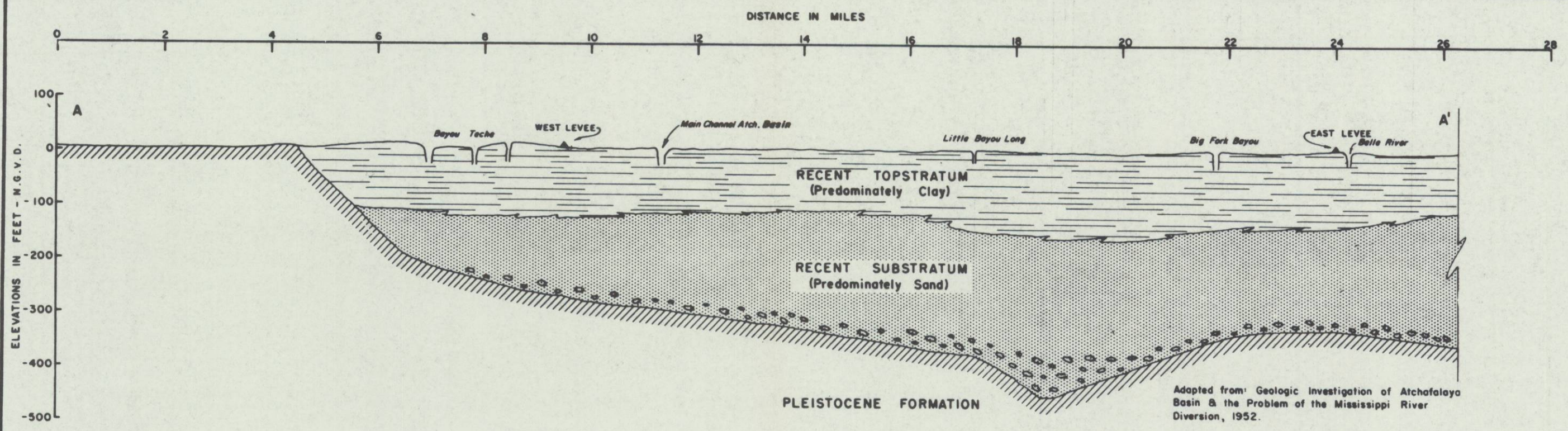
GENERALIZED GEOLOGIC CROSS SECTION A-A'
