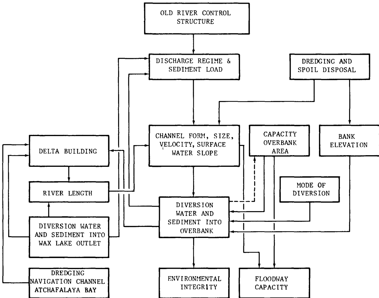
Figure 5. Relationships among hydraulic elements in the Atchafalaya Basin floodway system.
